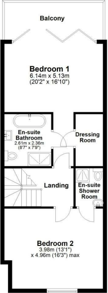
First Floor Approx. 61.3 sq. metres (660.0 sq. feet)
